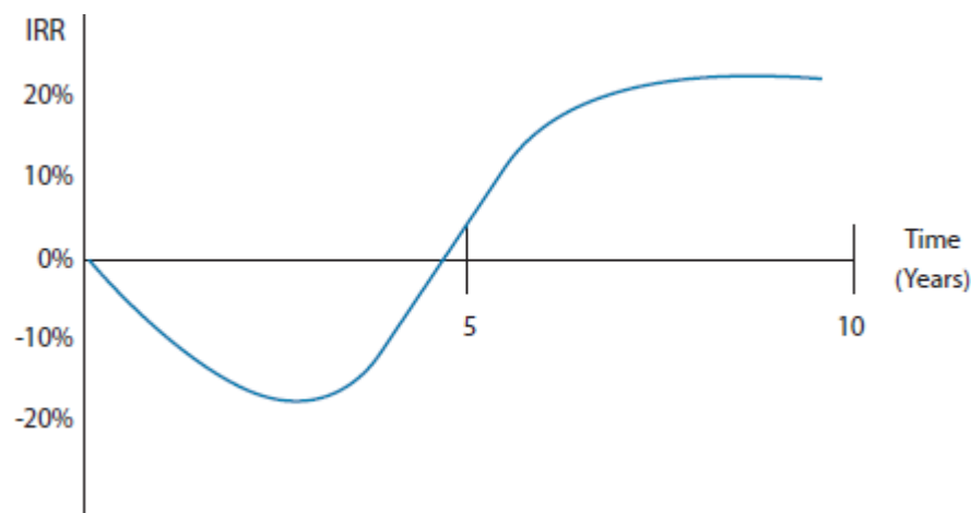
Figure 77.1: J-Curve Example
